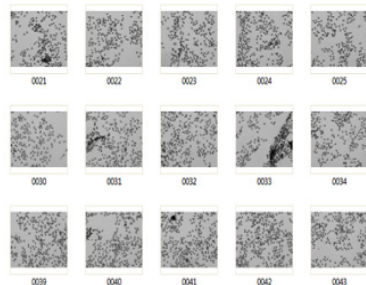
DNA staining
