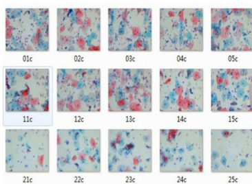
Pap staining
