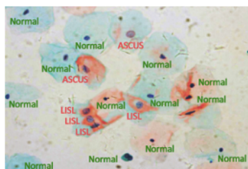
Morphological analysis
