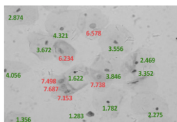
Quantitative analysis
